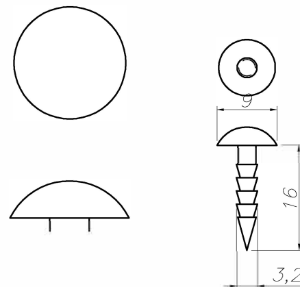
PG9X3,2X16R/NI
