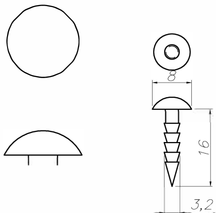
PG8X3,2X16R/NI
